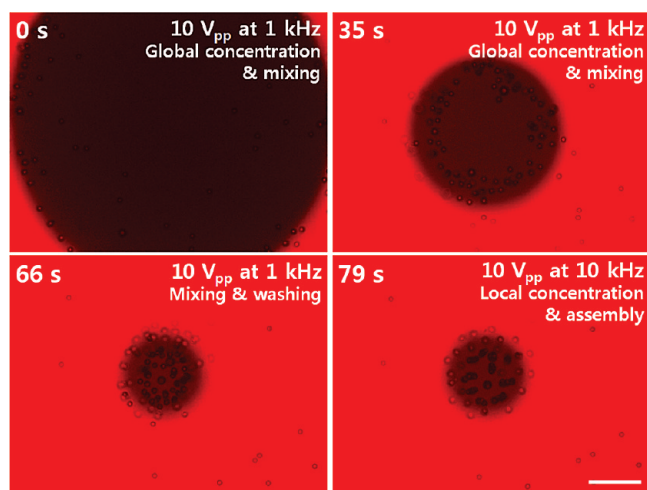
Figure 2. Microscopic pictures of PS microspheres being processed for optoelectrofluidic immunoassay. At 1 kHz, an animated LCD image concentrates the microspheres by ACEO vortices and negative DEP forces. After the animation stops, the strong ACEO flows mix the concentrated microspheres with target analytes and probe nanoparticles, and wash free molecules and nanoparticles from the dark area. At 10 kHz, the washed immunocomplexes are assembled and concentrated into the area for detection of SERS. Scale bar = 25 \mu\text{m} .
