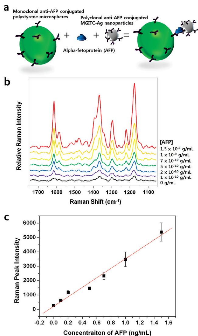
Figure 5. The quantitative assay of human AFP based on optoelectrofluidic SERS. (a) Schematic illustration of the formation of immunocomplex for SERS-based assay. Human AFP and MGITC-tagged AgNPs were applied for target analytes and probe nanoparticles, respectively. (b) SERS spectra for various concentrations of AFP antigen. (c) Intensity of the SERS signal at 1615 cm -1 against the concentration of AFP. A linear relationship is shown in the concentration range from 0 to 1.5 ng/mL. The linear fitting line is y = 3302x + 216.9 , and R = 0.9910 ( n = 6 ).
